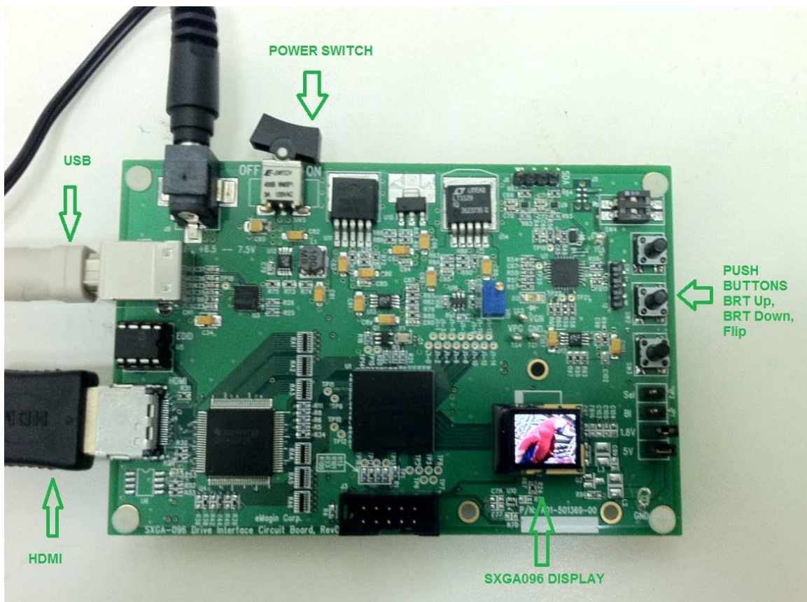
Figure 3-1 SXGA096 Design Reference Board
