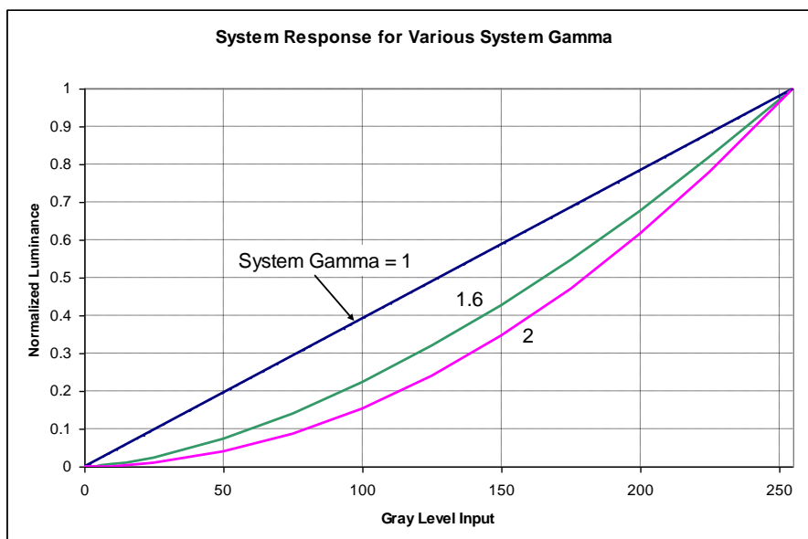
Figure 25 : Display system response for arbitrary system gamma
