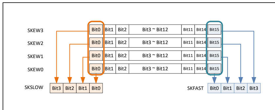
Figure 39 : SKFAST and SKSLOW register mapping
