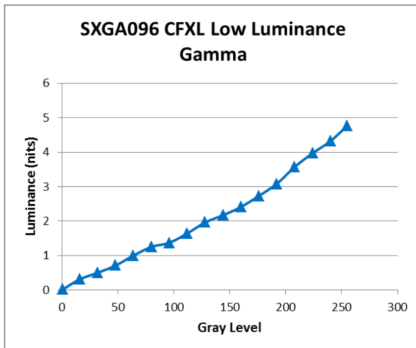
Figure 23: Low Luminance Gamma Response
