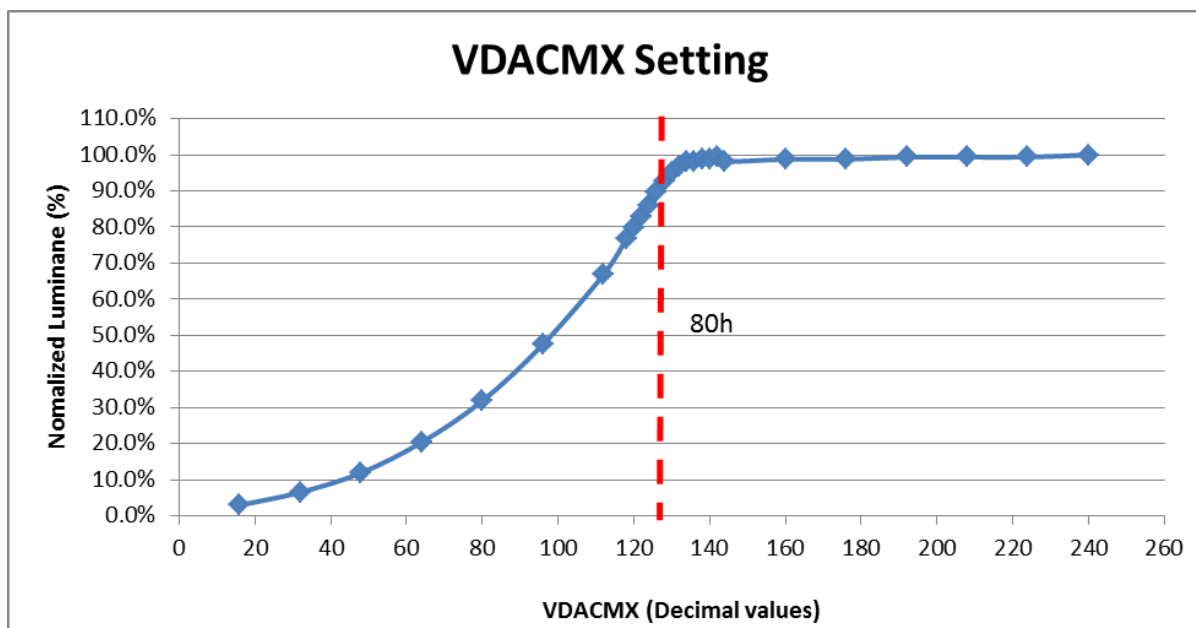
Figure 31: Luminance dependency on VDACMX
