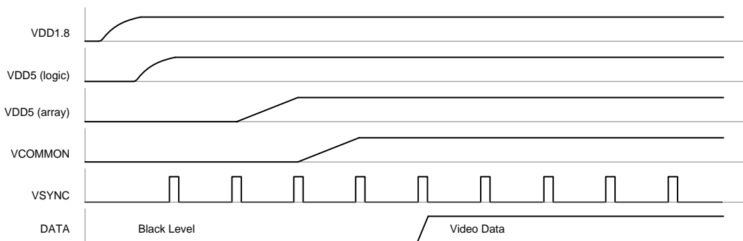
Figure 28 : Power-Up sequence for supplies and control.
