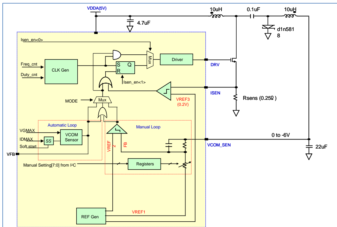
Figure 26 : Schematic of DC-DC controller function
