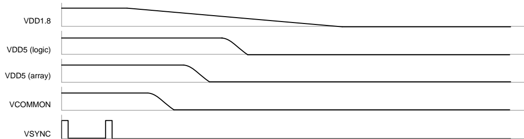
Figure 29 : Power-Down sequence for supplies and control.
