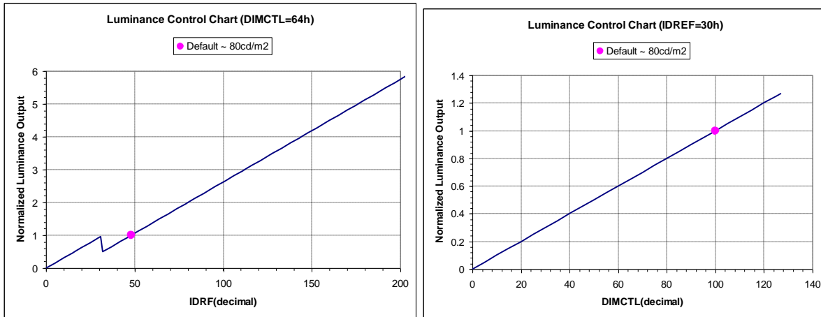
Figure 19: luminance profile for various IDRf settings
