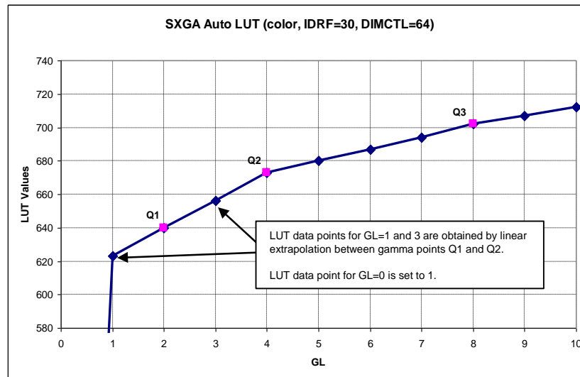
Figure 21 : Gamma curve at low gray levels
