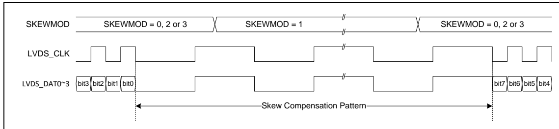
Figure 37 : Skew compensation pattern
