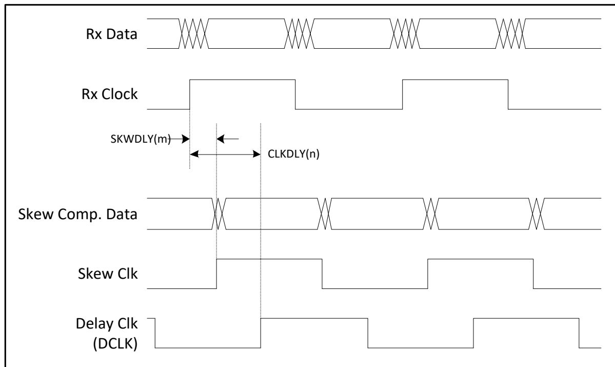
Figure 34 : LVDS Skew compensation timing diagram
