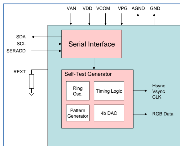
Figure 30 : Block diagram of setup for BI mode
