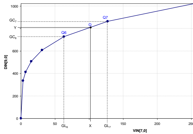
Figure 20 : Generating intermediate points by linear interpolation
