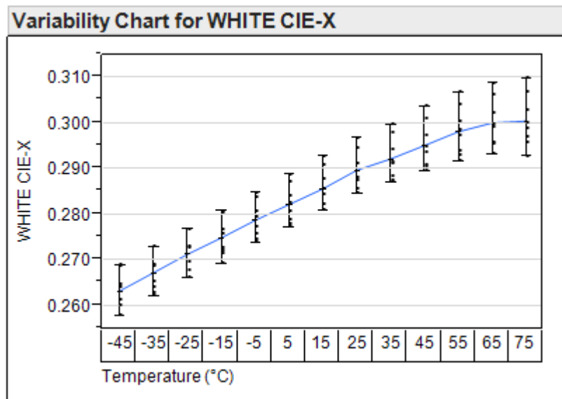
Figure 10: White CIE-X vs. Temperature @ 150 cd/m 2
