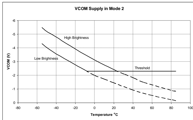
Figure 27 : VCOM supply characteristic in Mode 2
