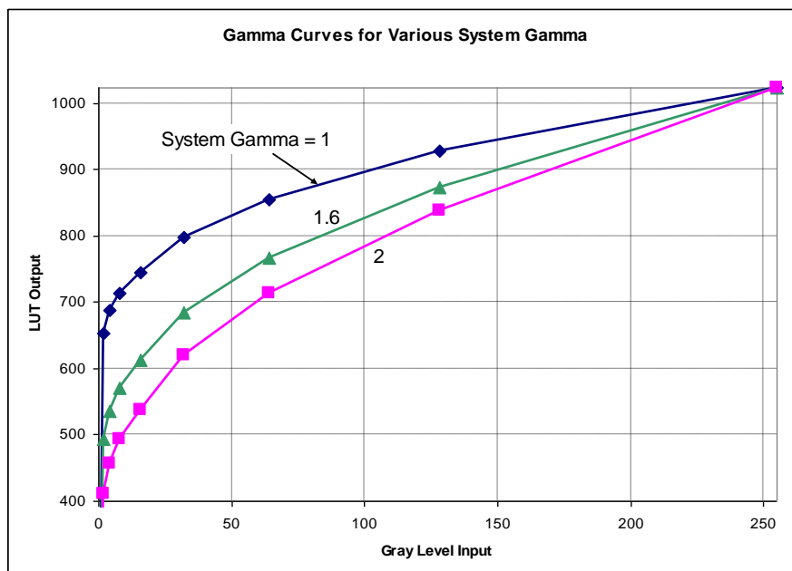
Figure 24 : Gamma curves for arbitrary System Gamma
