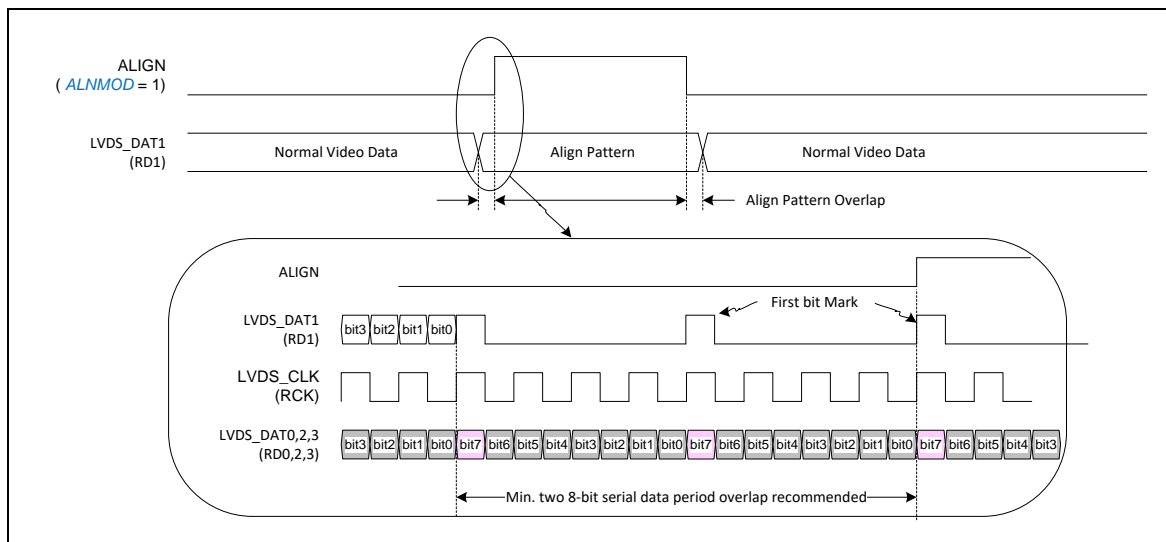
Figure 35 : LVDS Align pattern
