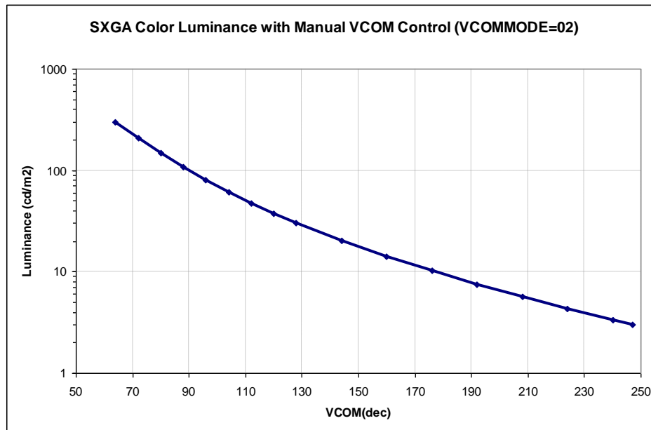
Figure 32 : Typical luminance dependency on manual VCOM setting
