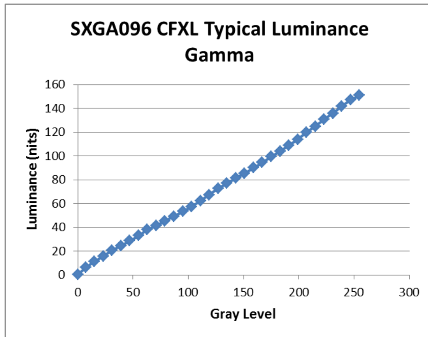
Figure 22: Typical Luminance Gamma Response
