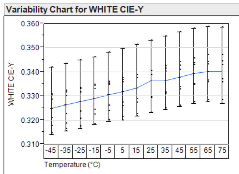
Figure 11: White CIE-Y vs. Temperature @ 150 cd/m 2
