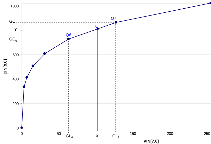
Figure 26 : Generating intermediate points by linear interpolation
