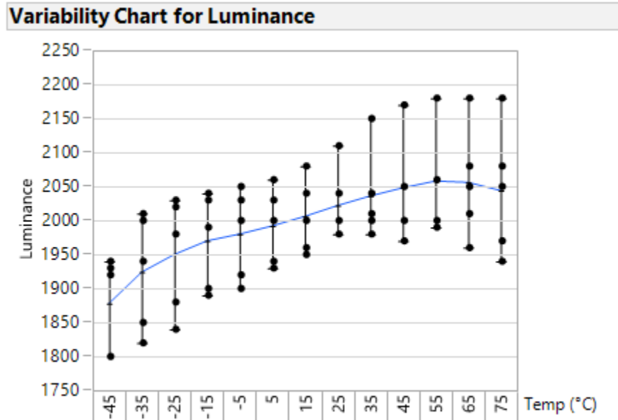
Figure 14: Luminance stability vs. Temperature
