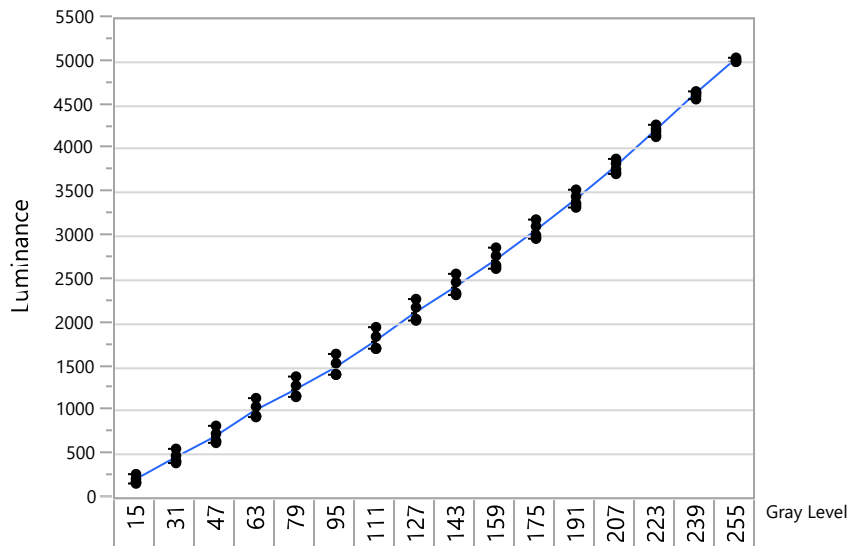
Figure 13: SXGA096 MGXLT Luminance vs. Gray Level
