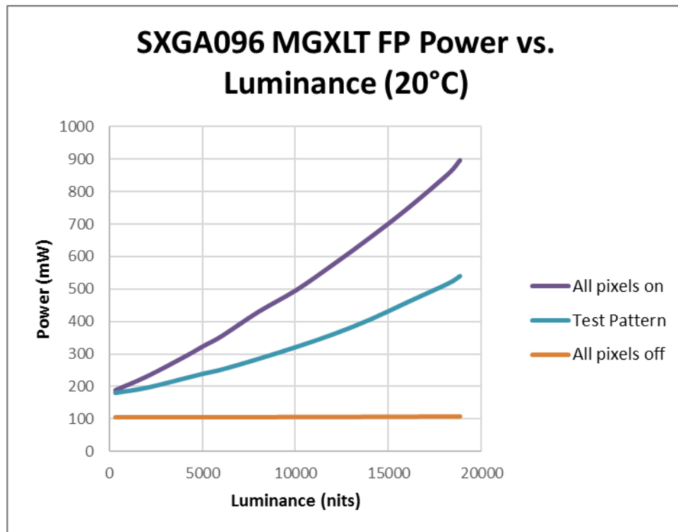
Figure 6: SXGA096 MGXLTFP Power vs. Luminance
