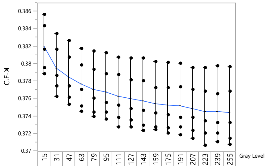
Figure 11: SXGA096 MGCLT CIE-X vs. Graylevel (@5,000 cdm -2 )
