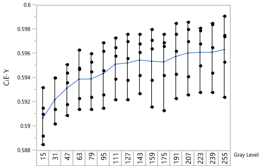
Figure 12: SXGA096 MGXLT CIE-Y vs. Gray Level (@ 5,000 cdm -2 )
