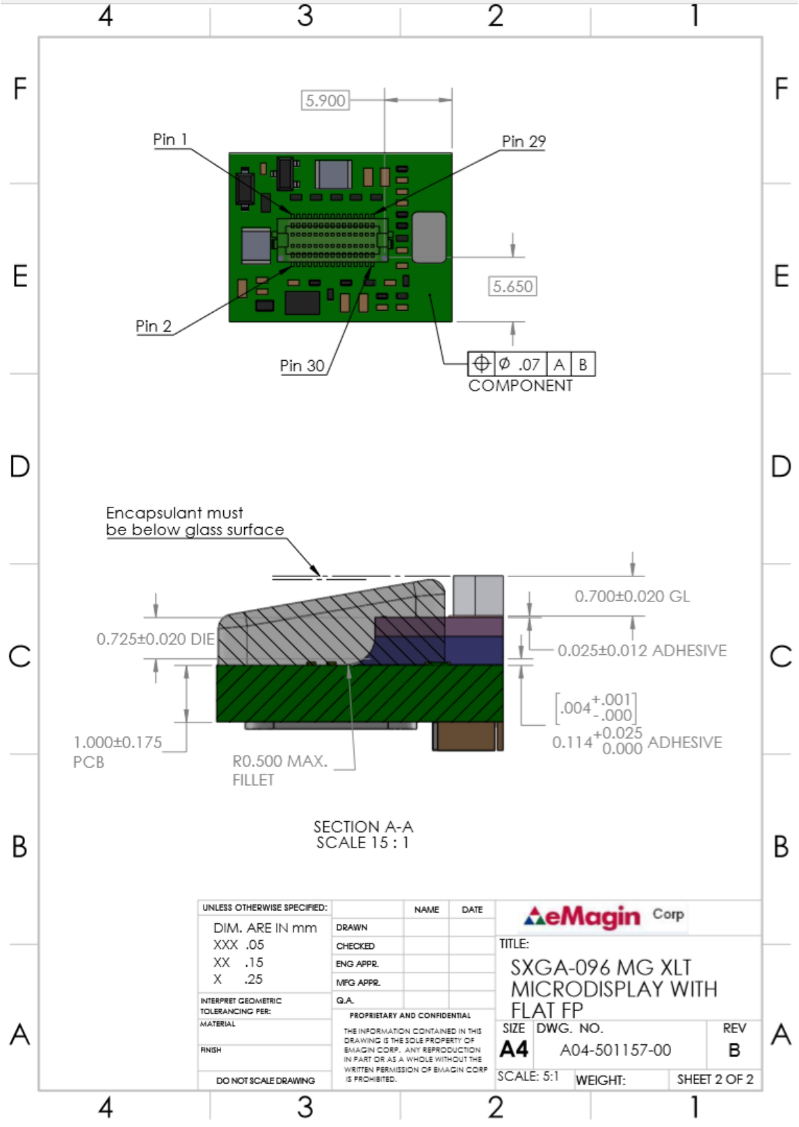
Figure 18: SXGA-096 Microdisplay Assembly - Detail
