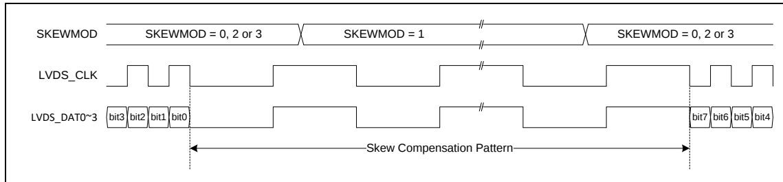
Figure 42 : Skew compensation pattern
