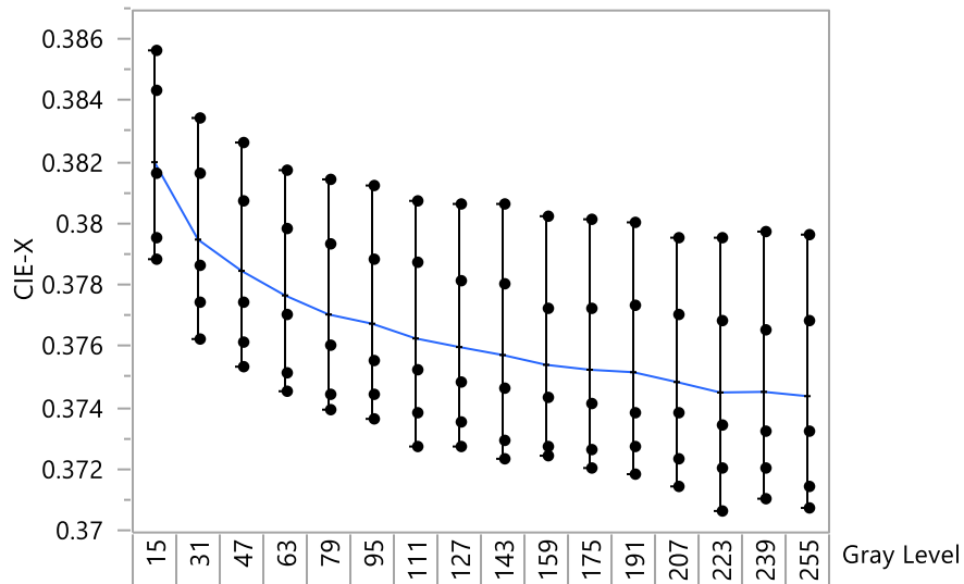
Figure 11: SXGA096 MGCLT CIE-X vs. Graylevel (@5,000 cdm -2 )
