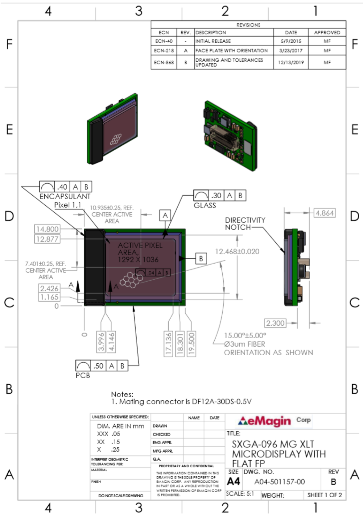
Figure 17: SXGA-096 MG XLT Microdisplay Assembly
