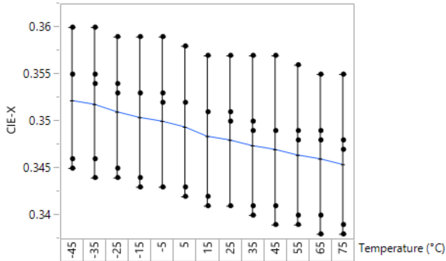
Figure 15: Green CIE-X vs. Temperature @ 5,000 cd/m 2
