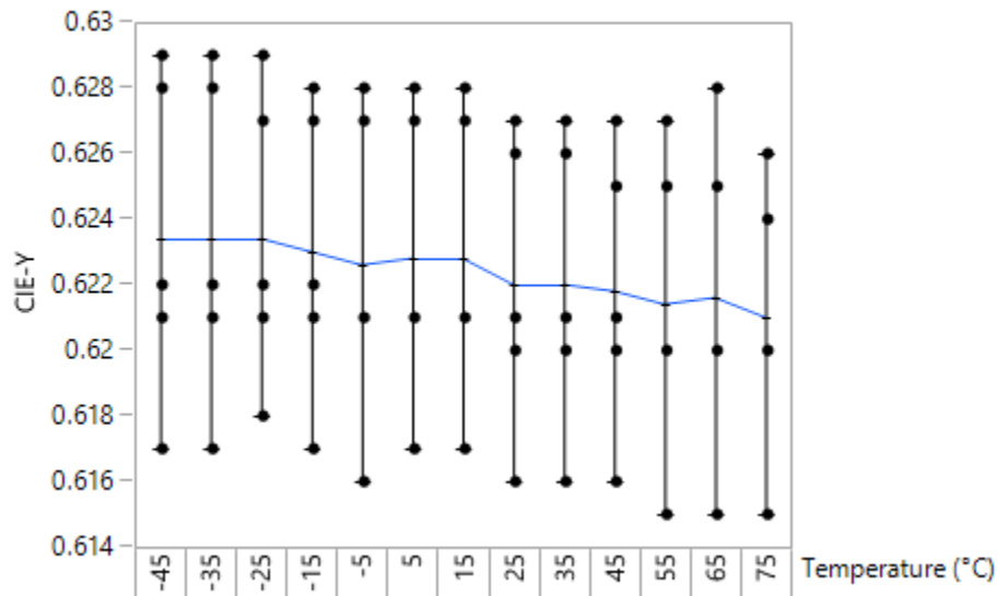
Figure 16: Green CIE-Y vs. Temperature @ 5,000 cd/m 2
