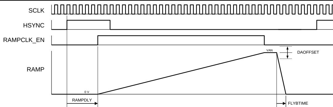
Figure 14 : Timing diagram for column data sampling
