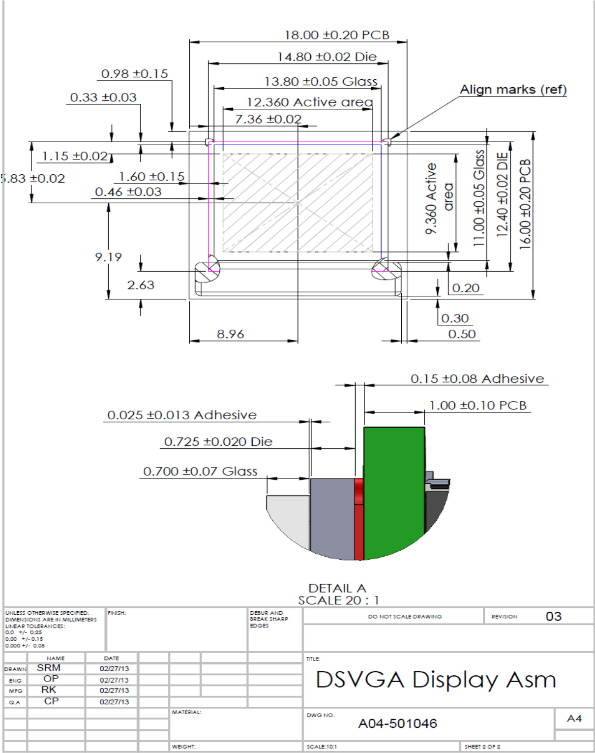
Figure 10: DSVGA Microdisplay Assembly Drawing
