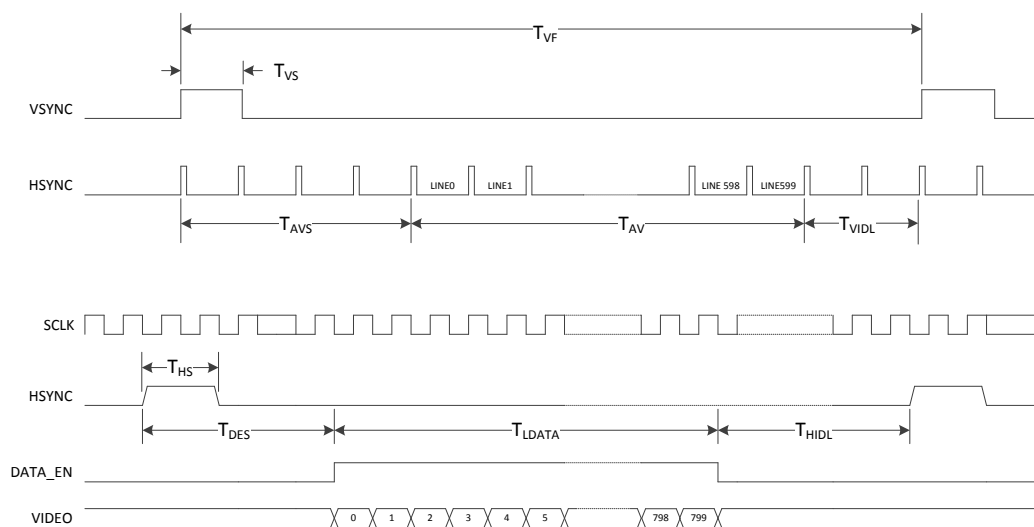
Figure 6: Line Timing
