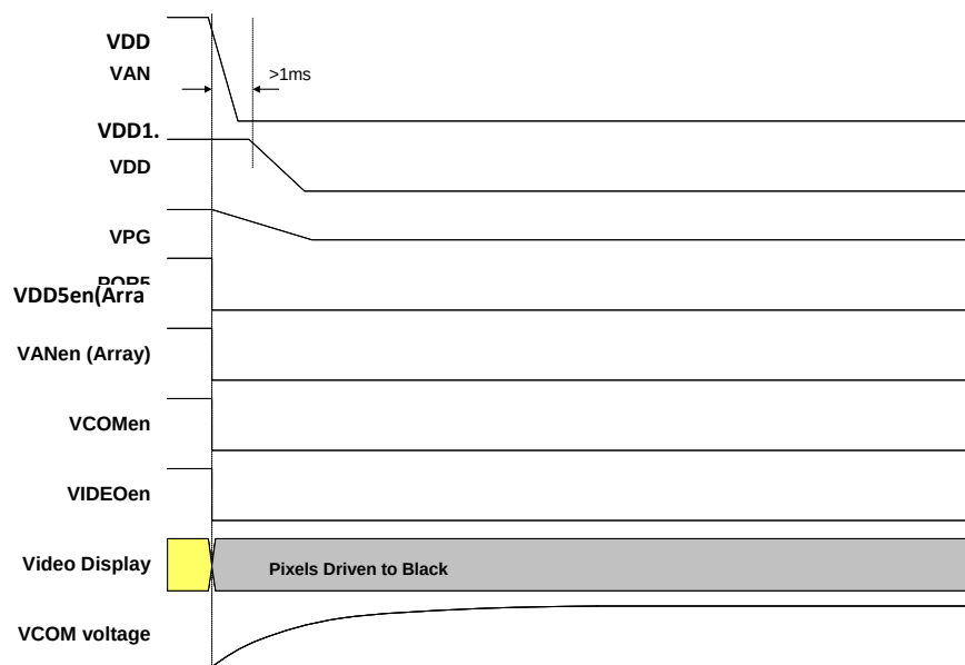
Figure 26: Power-Down sequence for supplies and control.
