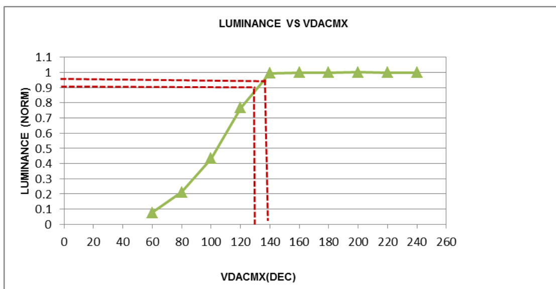
Figure 28: Luminance dependency on VDACMX
