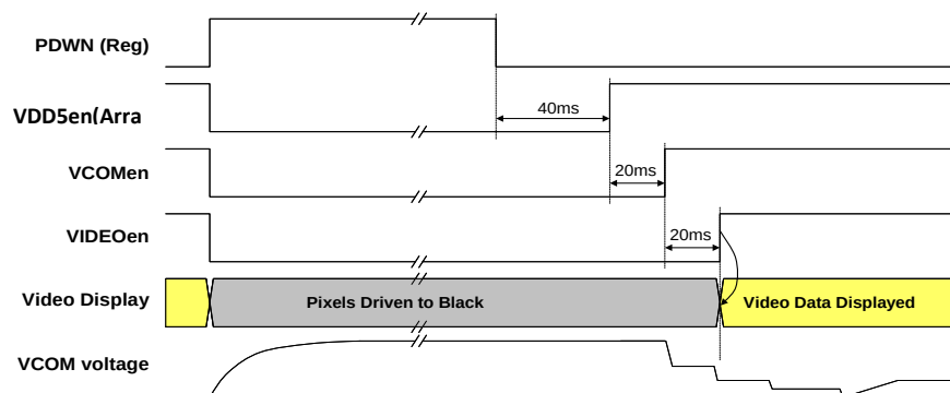
Figure 27: Soft power-down / power-on sequence for supplies and control.
