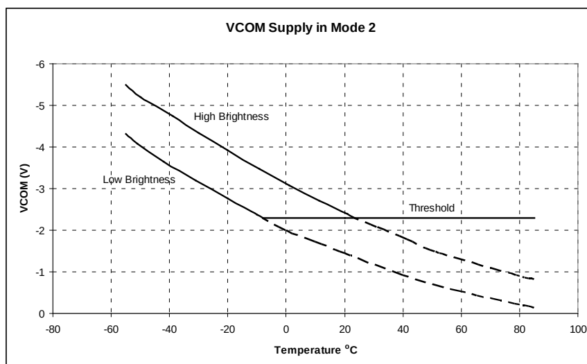
Figure 23: VCOM supply characteristic in Mode 2
