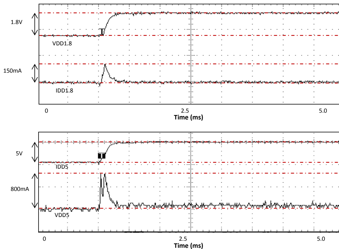
Figure 25: Typical startup currents
