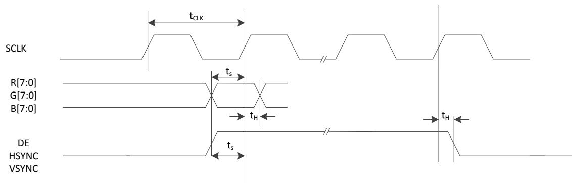
Figure 5: Pixel Timing
