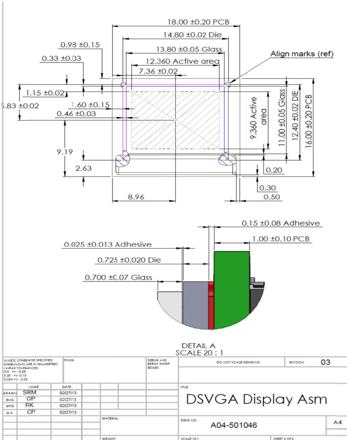
Figure 3: DSVGA Microdisplay Assembly Drawing
